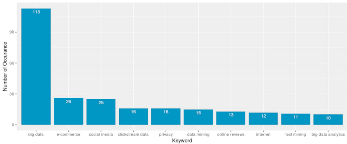
Fig. 4. Keyword occurrence.
