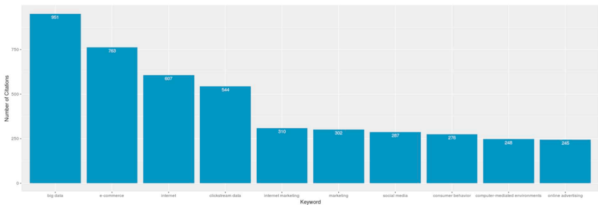
Fig. 5. Keyword citations.
